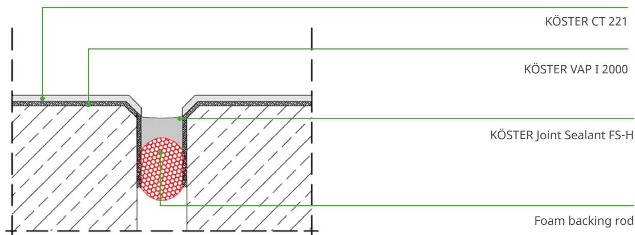
Cracks and dilation joints
