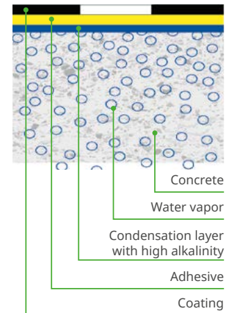
Development of high alkalinity
