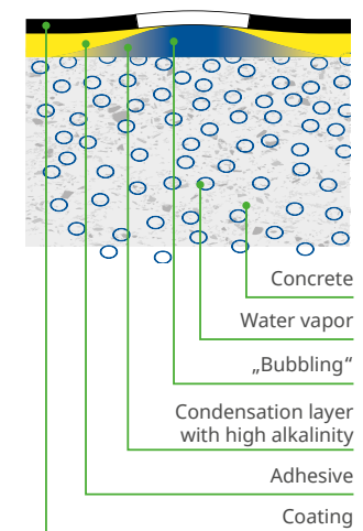
Formation of "osmotic bubbles"
